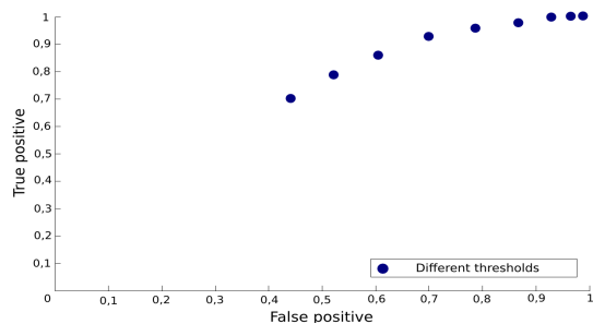
Fig. 4. Evaluation of the original algorithm [7] with different thresholds for speed change of 5% on ID_303
